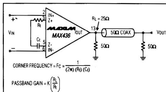
Figure 10. Highpass Amplifier
