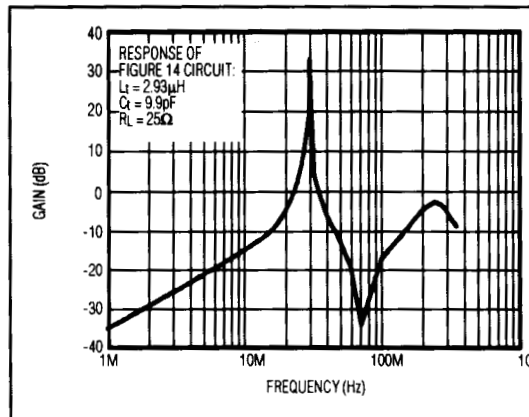
Figure 15. Tuned Amplifier Gain vs. Frequency
