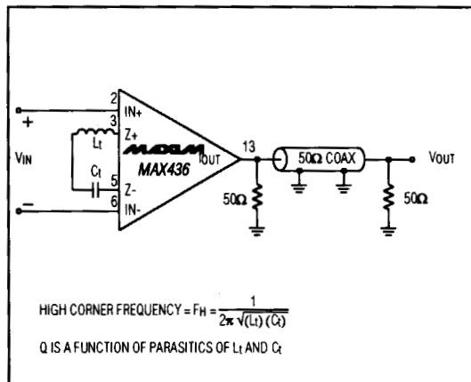
Figure 14. Tuned Amplifier
