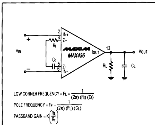
Figure 12. Bandpass Amplifier
