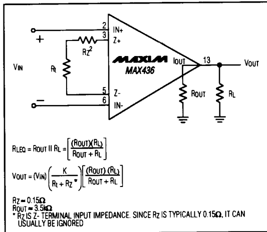
Figure 2. Finite Output-Impedance of WTA
